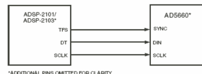
Figure 26. AD5660 to ADSP-2101/ADSP-2103 Interface
