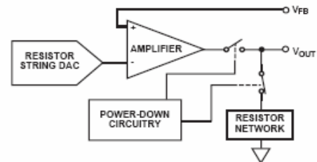
Figure 25. Output Stage During Power-Down
