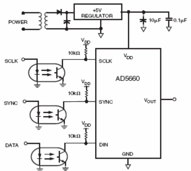
Figure 33. AD5660 with an Opto-Isolated Interface
