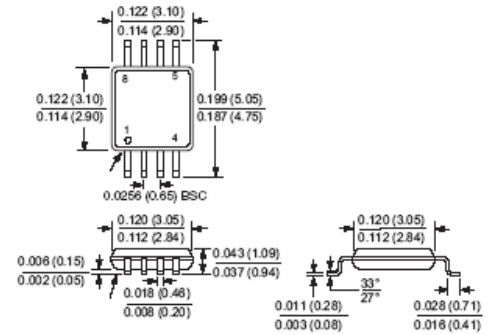
Figure 35. 8-Lead MSOP (RJ-8)
