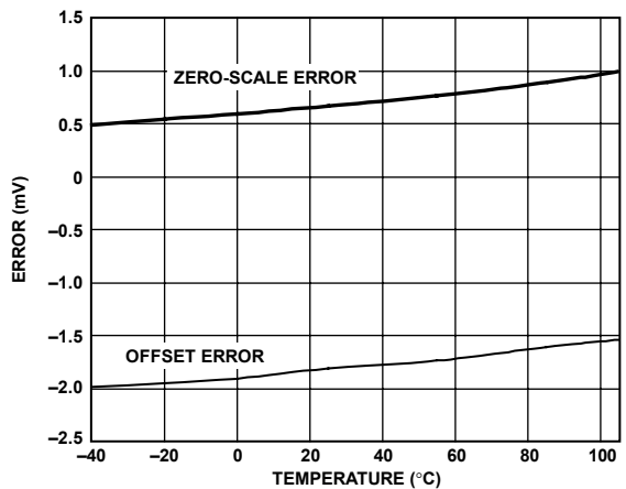
Figure 18. Zero-Scale Error and Offset Error vs. Temperature
