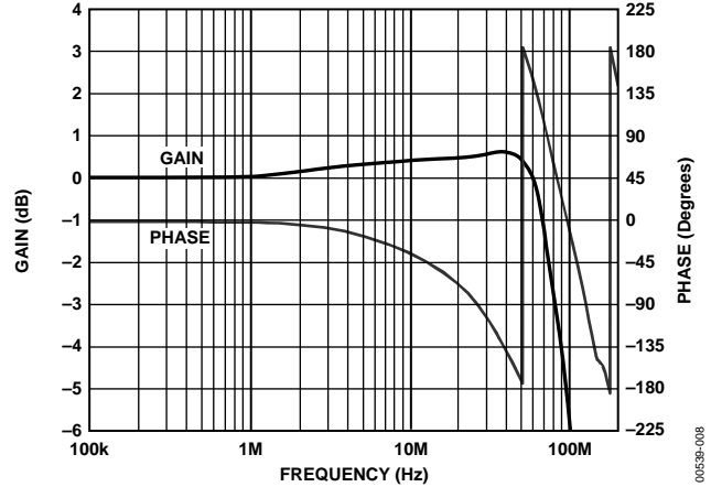
Figure 8. Frequency and Phase Response vs. Gain (Gain = +30\text{ dB} , P_{IN} = -30\text{ dBm} )
