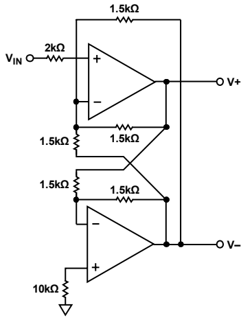
Figure 45. Single-Ended-to-Differential Configuration with the AD845 for Bipolar Operation
