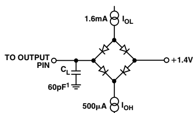
Figure 1. Load Circuit for Digital Interface Timing, SDOUT , SYNC , SCLK Outputs, C_L = 10\text{ pF}
