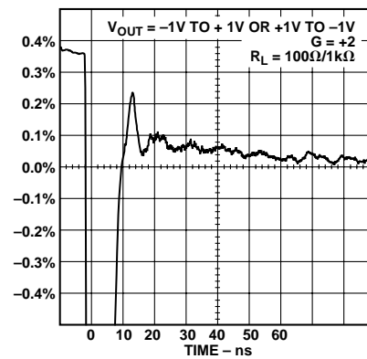
Figure 26. Settling Time
