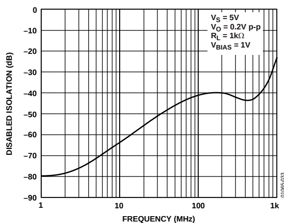
Figure 33. Disabled Output Isolation Frequency Response
