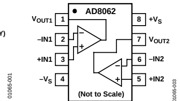
Figure 2. 8-Lead SOIC (R)/MSOP (RM)
