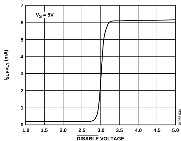
Figure 34. \overline{\text{DISABLE}} Voltage vs. Supply Current
