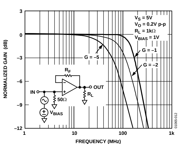
Figure 12. Small Signal Frequency Response
