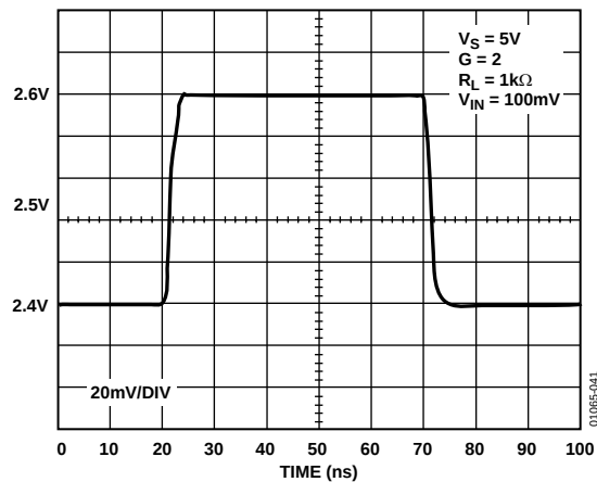
Figure 41. 100 mV Step Response
