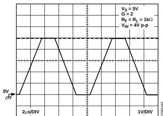
Figure 42. Output Rail-to-Rail Swing
