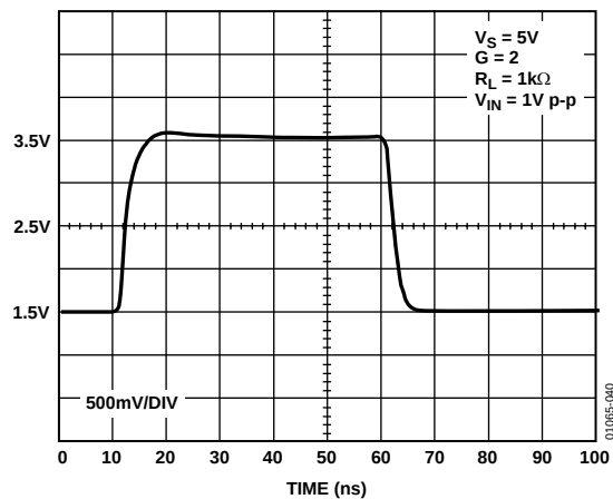
Figure 40. 1 V Step Response
