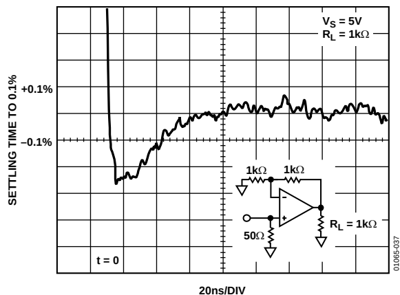
Figure 37. Output Settling Time to 0.1%
