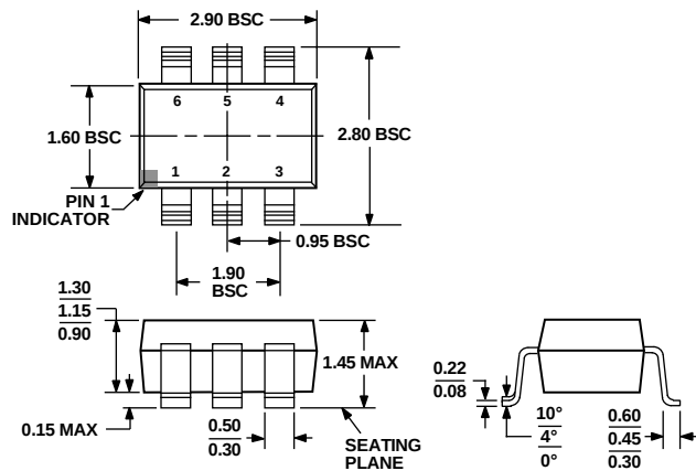
Figure 60. 6-Lead Small Outline Transistor Package [SOT-23] (RT-6) Dimensions shown in millimeters
