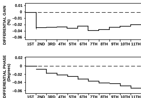
Figure 22. Differential Gain and Phase Error, G = 2 , NTSC Input Signal, R_L = 1k\Omega , V_S = 5V
