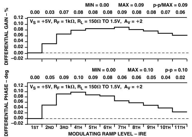
Figure 8. Differential Gain and Phase, V_S = +5V
