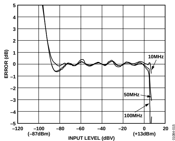
Figure 7. Log Linearity of RSSI Output vs. Input Level, at T_A = 25^\circ\text{C} , for Frequencies of 10 MHz, 50 MHz, and 100 MHz
