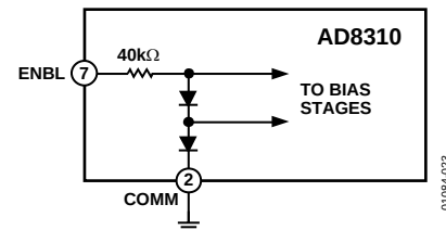
Figure 23. Enable Interface
