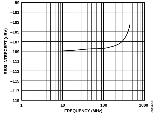
Figure 19. RSSI Intercept vs. Frequency
