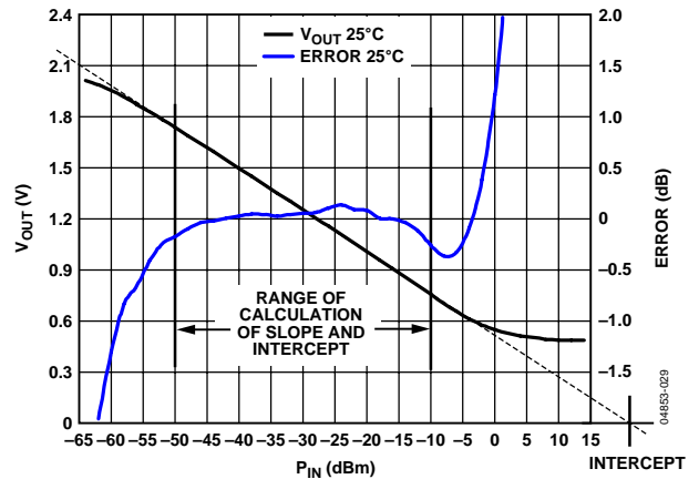
Figure 30. Typical Output Voltage vs. Input Signal
