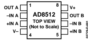
Figure 1. 8-Lead MSOP (RM Suffix)
