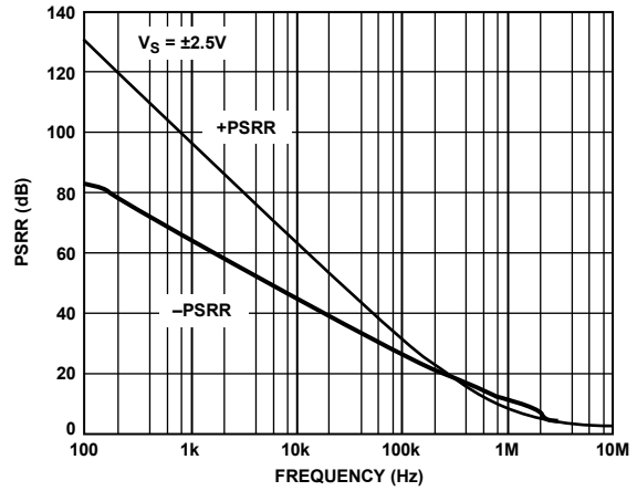
Figure 35. PSRR vs. Frequency at \pm 2.5V
