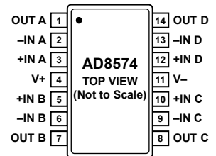
Figure 5. 14-Lead TSSOP (RU Suffix)
