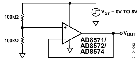
Figure 62. AD857x Test Circuit for Turn-On Time
