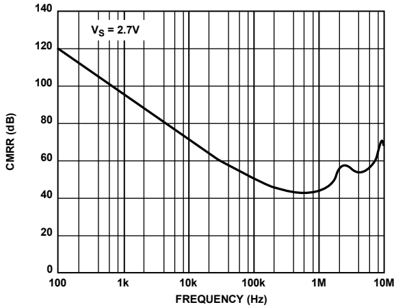
Figure 32. CMRR vs. Frequency at 2.7 V
