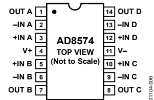
Figure 6. 14-Lead SOIC (R Suffix)
