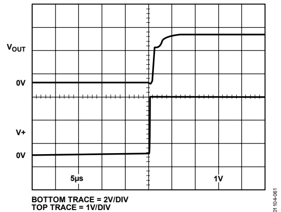
Figure 61. AD857x Output Behavior on Power-Up
