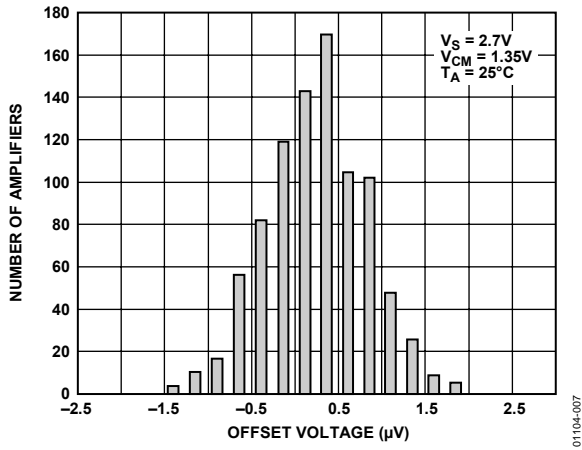
Figure 7. Input Offset Voltage Distribution at 2.7 V
