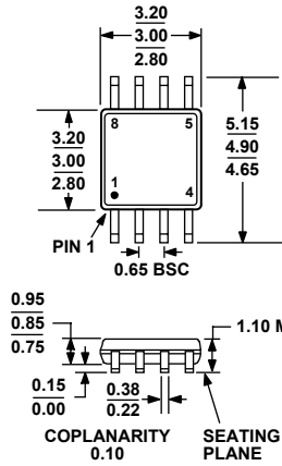
Figure 27. 8-Lead Mini Small Outline Package [MSOP] (RM-8)
