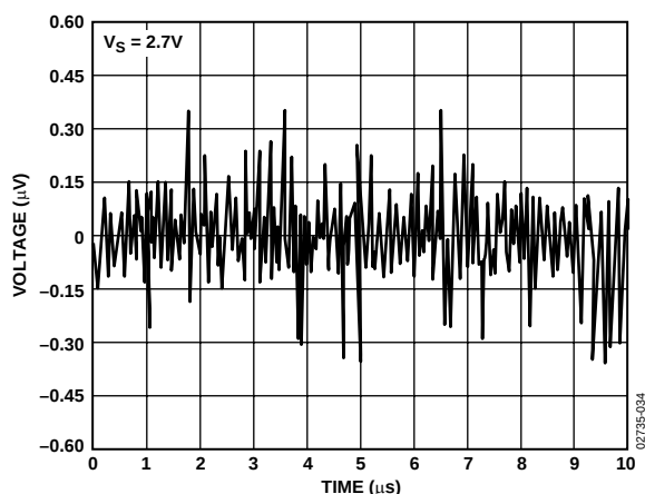
Figure 38. 0.1 Hz to 10 Hz Noise
