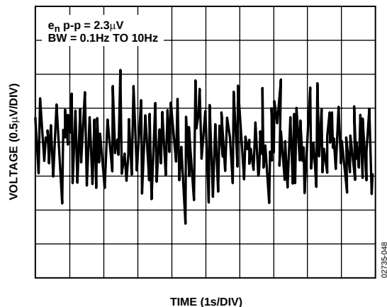
Figure 53. LTC2050 Peak-to-Peak Noise
