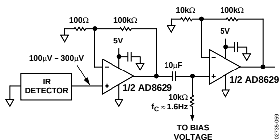
Figure 64. AD8629 Used as Preamplifier for Thermopile
