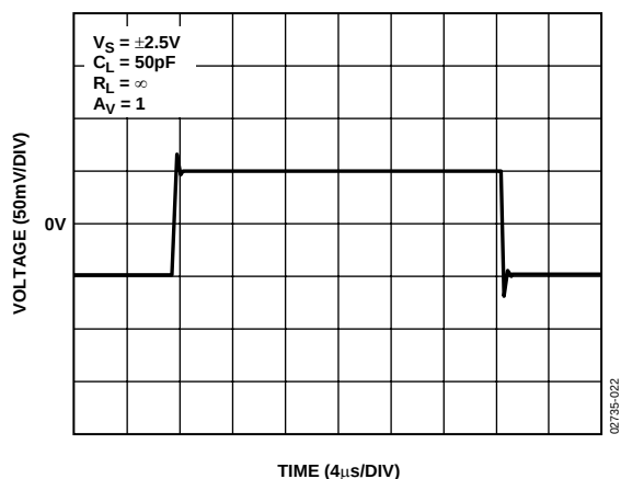
Figure 26. Small Signal Transient Response
