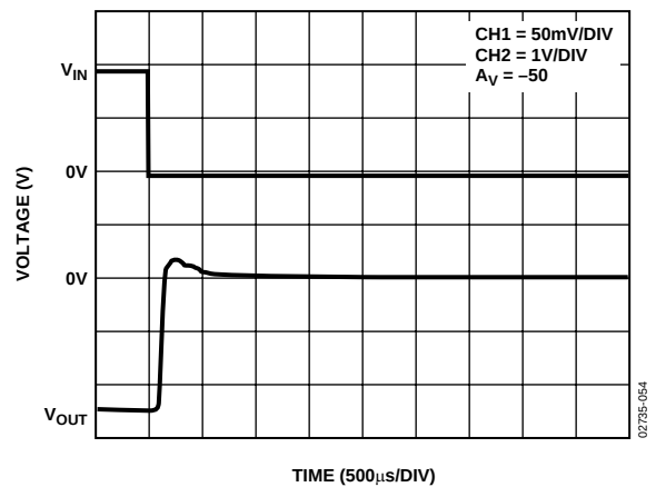
Figure 59. Positive Input Overload Recovery for LTC2050
