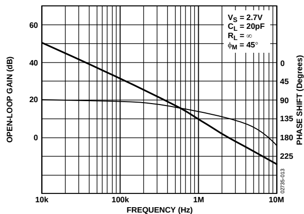
Figure 17. Open-Loop Gain and Phase vs. Frequency
