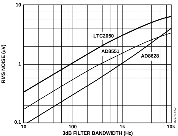
Figure 57. 3 dB Filter Bandwidth in Hz
