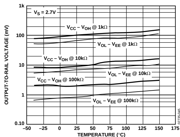
Figure 49. Output-to-Rail Voltage vs. Temperature
