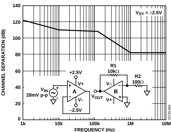
Figure 50. AD8629/AD8630 Channel Separation
