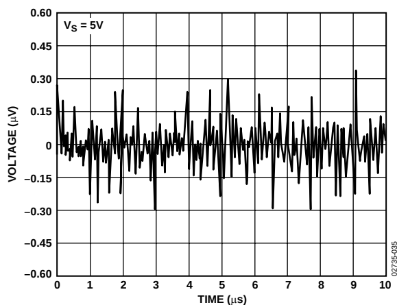
Figure 39. 0.1 Hz to 10 Hz Noise
