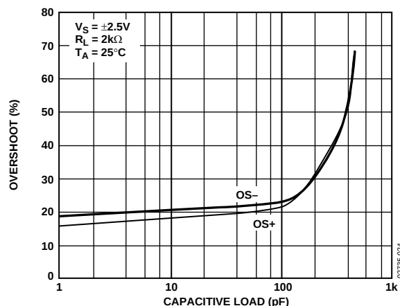
Figure 28. Small Signal Overshoot vs. Load Capacitance
