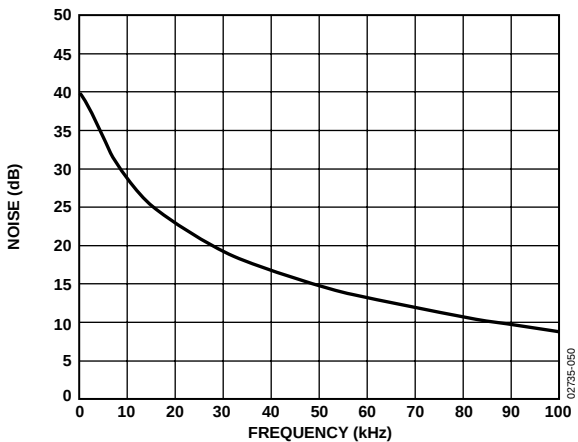
Figure 55. Simulation Transfer Function of the Test Circuit
