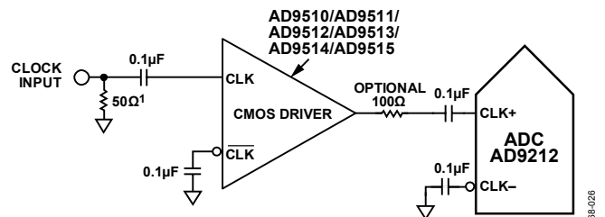
Figure 55. Single-Ended 3.3 V CMOS Sample Clock
