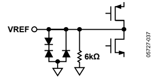
Figure 14. Equivalent VREF Circuit
