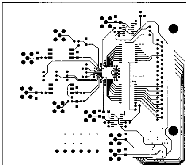
Figure 27. Printed Circuit Board Top Side Copper
