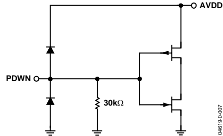
Figure 7. Power-Down Input
