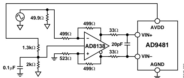
Figure 29. Driving the ADC with the AD8138
