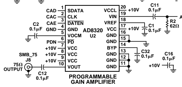
Figure 39. Electrical Schematic of AD9853-xxPCB Evaluation Board
