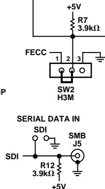
Figure 39. Electrical Schematic of AD9853-xxPCB Evaluation Board
