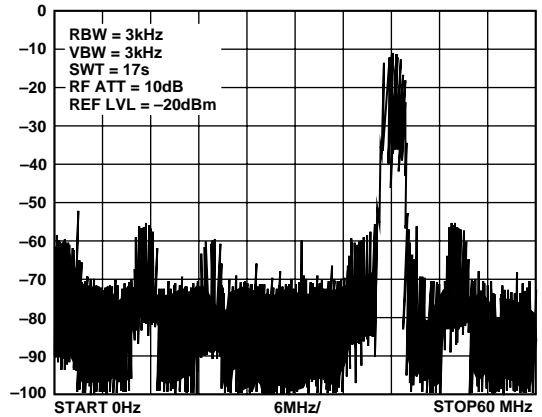
Figure 6. QPSK, 5.12 Mb/s, A_{OUT} = 42 MHz
