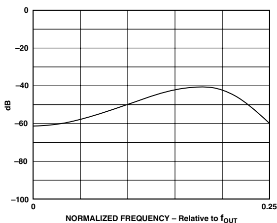
Figure 13d. Passband Frequency Response of the Decimator
