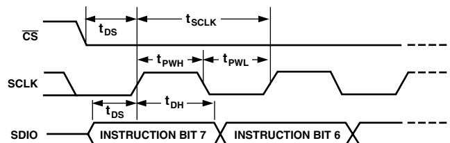
Figure 7. Timing Diagram for Register Write to AD9873
