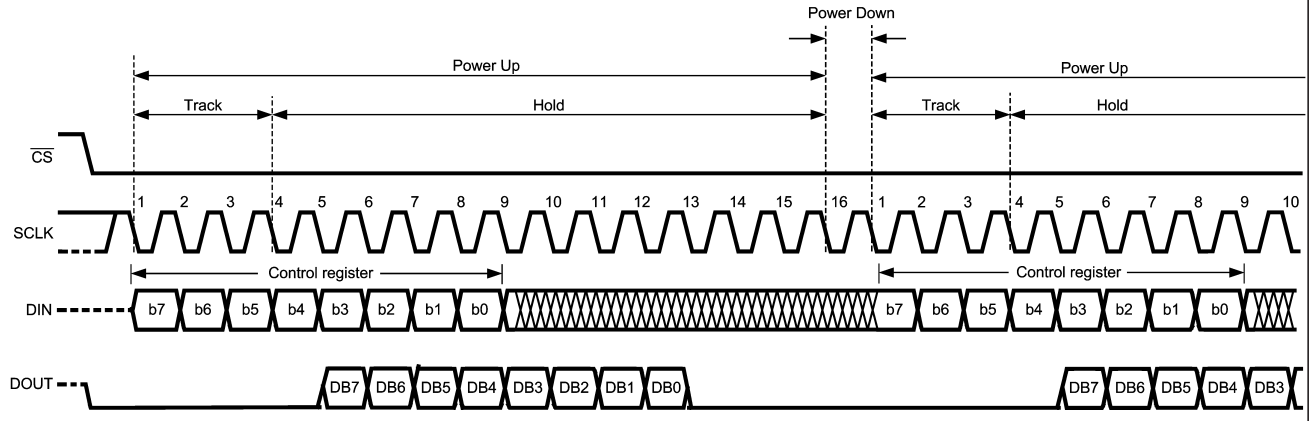
ADC082S021 Operational Timing Diagram
