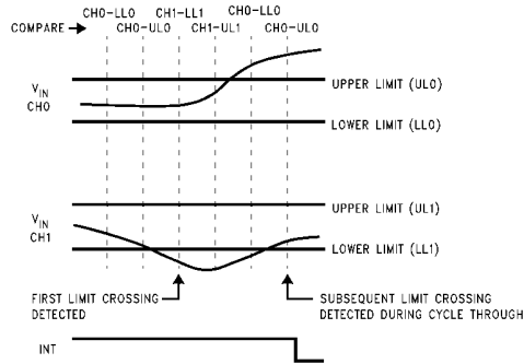
(Example: Lower limit of CH1 is crossed first. During cycle through, upper limit of CH0 is crossed)
