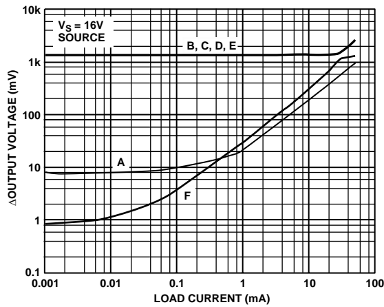
Figure 9. Output Source Voltage vs. Load Current, All Channels
