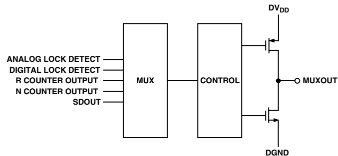
Figure 25. MUXOUT Circuit
