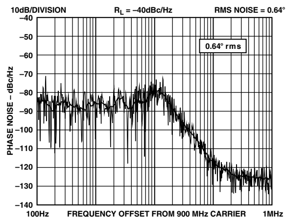
Figure 4. ADF4118 Integrated Phase Noise (900 MHz, 200 kHz, 35 kHz, Typical Lock Time: 200 \mu s)
