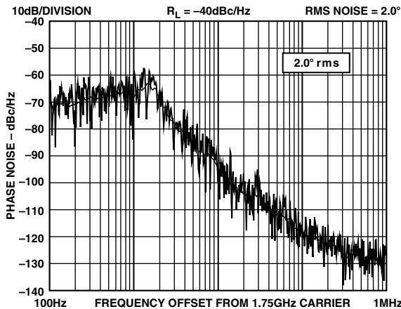
Figure 9. ADF4118 Integrated Phase Noise (1750 MHz, 30 kHz, 3 kHz)
