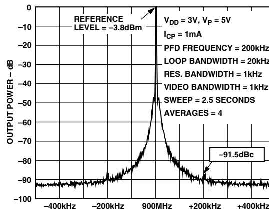
Figure 6. ADF4118 Reference Spurs (900 MHz, 200 kHz, 20 kHz)
