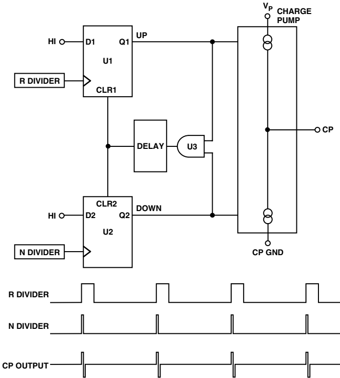
Figure 24. PFD Simplified Schematic and Timing (In Lock)
