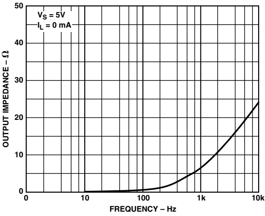
TPC 24. ADR292 Output Impedance vs. Frequency
