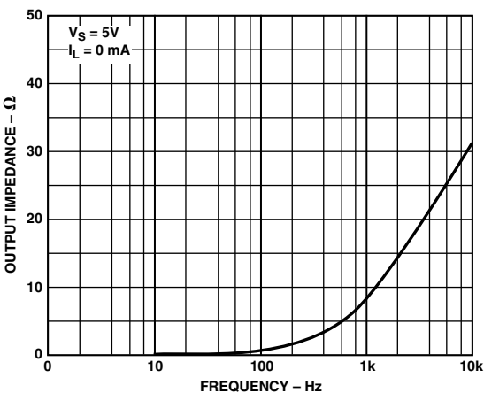
TPC 23. ADR291 Output Impedance vs. Frequency
