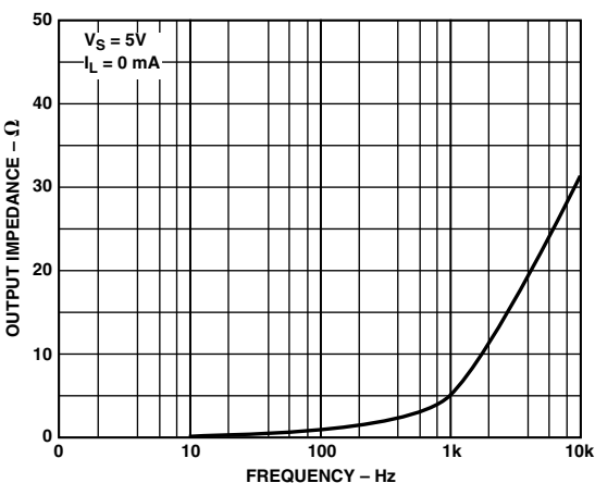
TPC 22. ADR290 Output Impedance vs. Frequency
