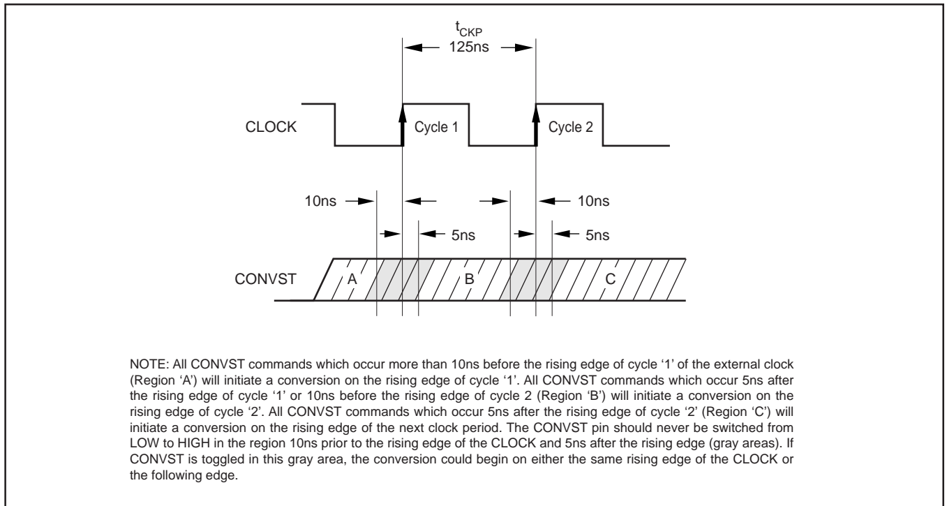
FIGURE 8. Conversion Mode.
