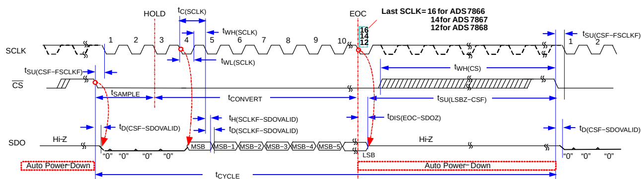
Figure 1. Timing Diagram
