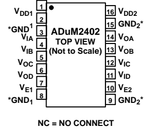
Figure 7. ADuM2402 Pin Configuration
