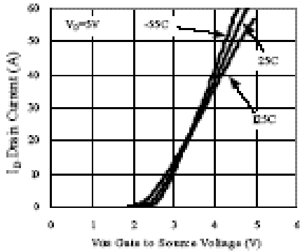
Figure 5. Transfer Characteristics
