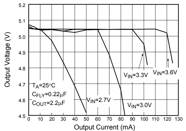
Fig. 4 Load Regulation
