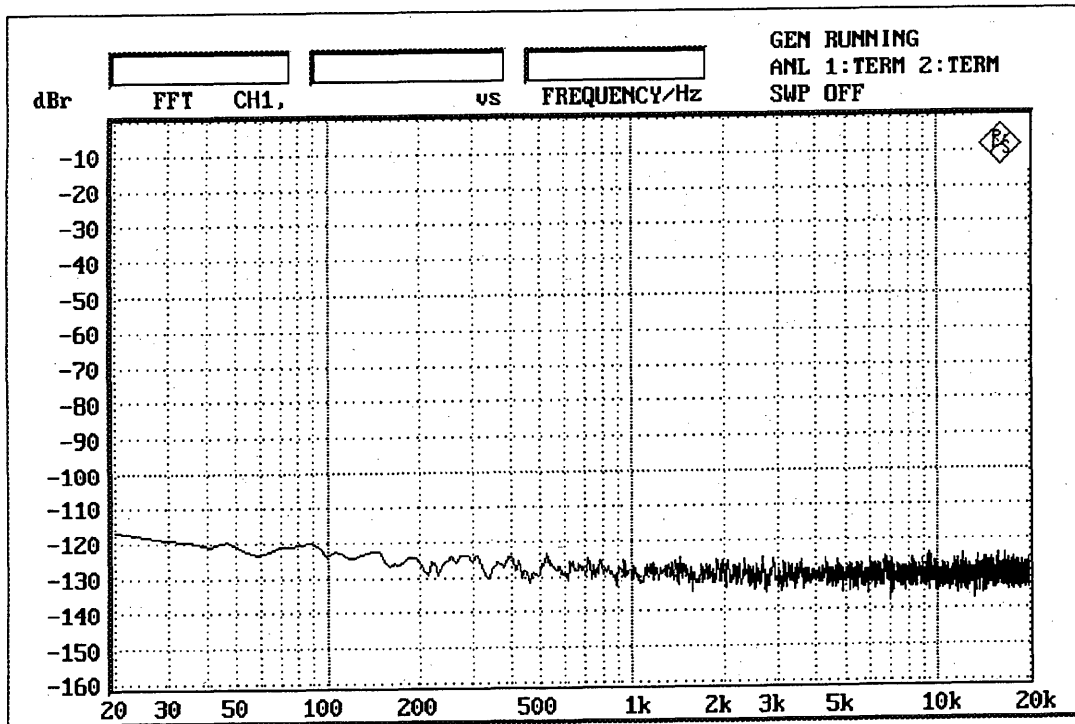
Figure 51 : FFT (noise floor ;
