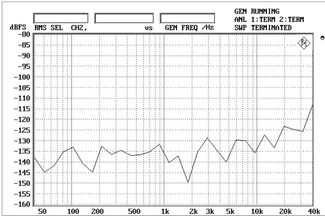
Fig.6 crosstalk
