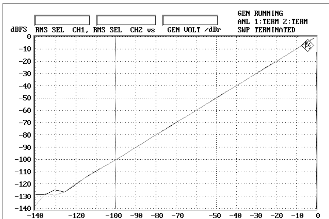
Fig.7 Linearity
