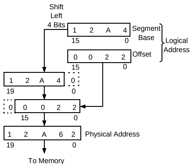
Figure 2. Two-Component Address
