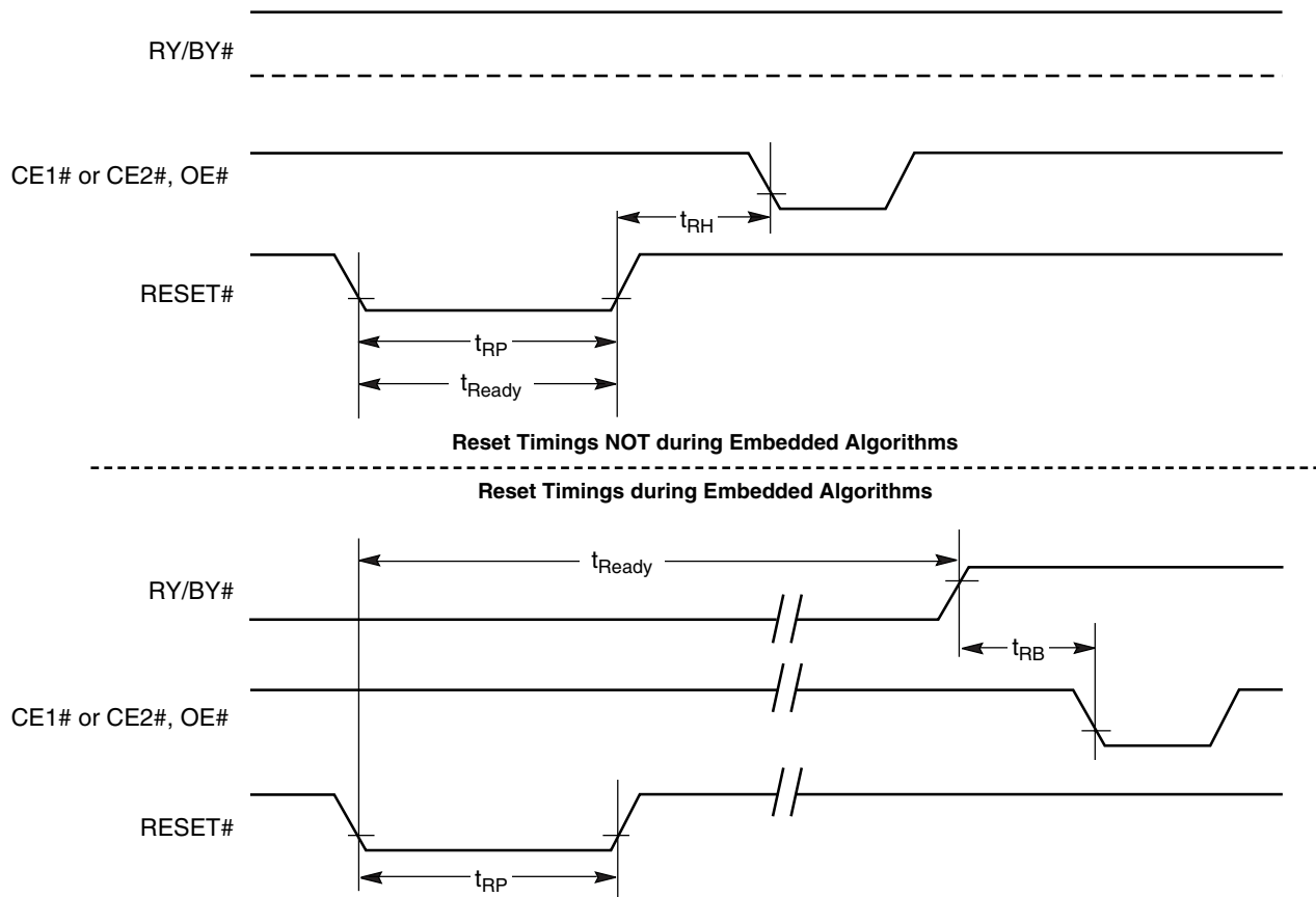
Figure 13. Reset Timings
