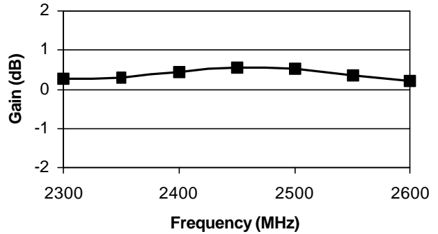
Gain, Low Power Mode
