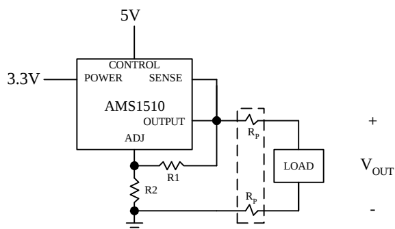
Figure 1. Conventional Load Sensing
