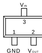
SOT-23 (Top View) APL5308
