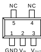
SOT-23-5 (Top View) APL5308
