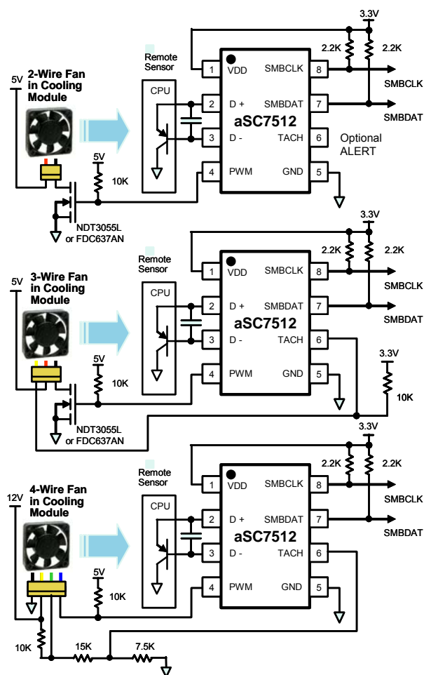
Figure 14 aSC7512 2-, 3- and 4-Wire Fan Connections
