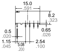
2 coil latching
