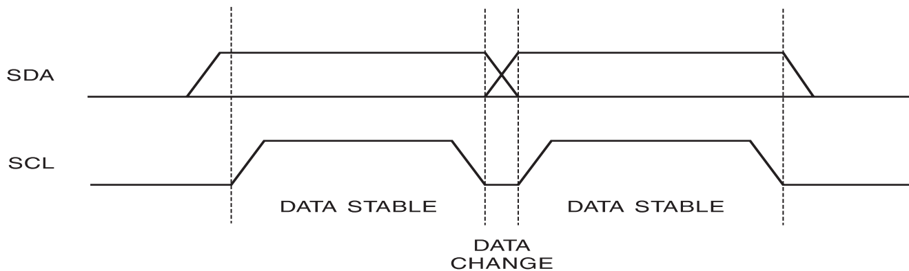
Figure 4. Data Validity
