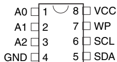
8-lead PDIP
