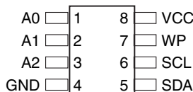
8-lead SOIC
