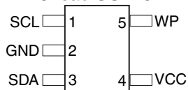
5-lead SOT23
