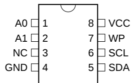
8-Pin PDIP
