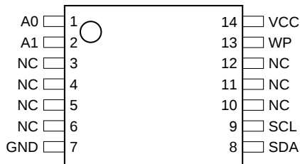
14-Pin TSSOP
