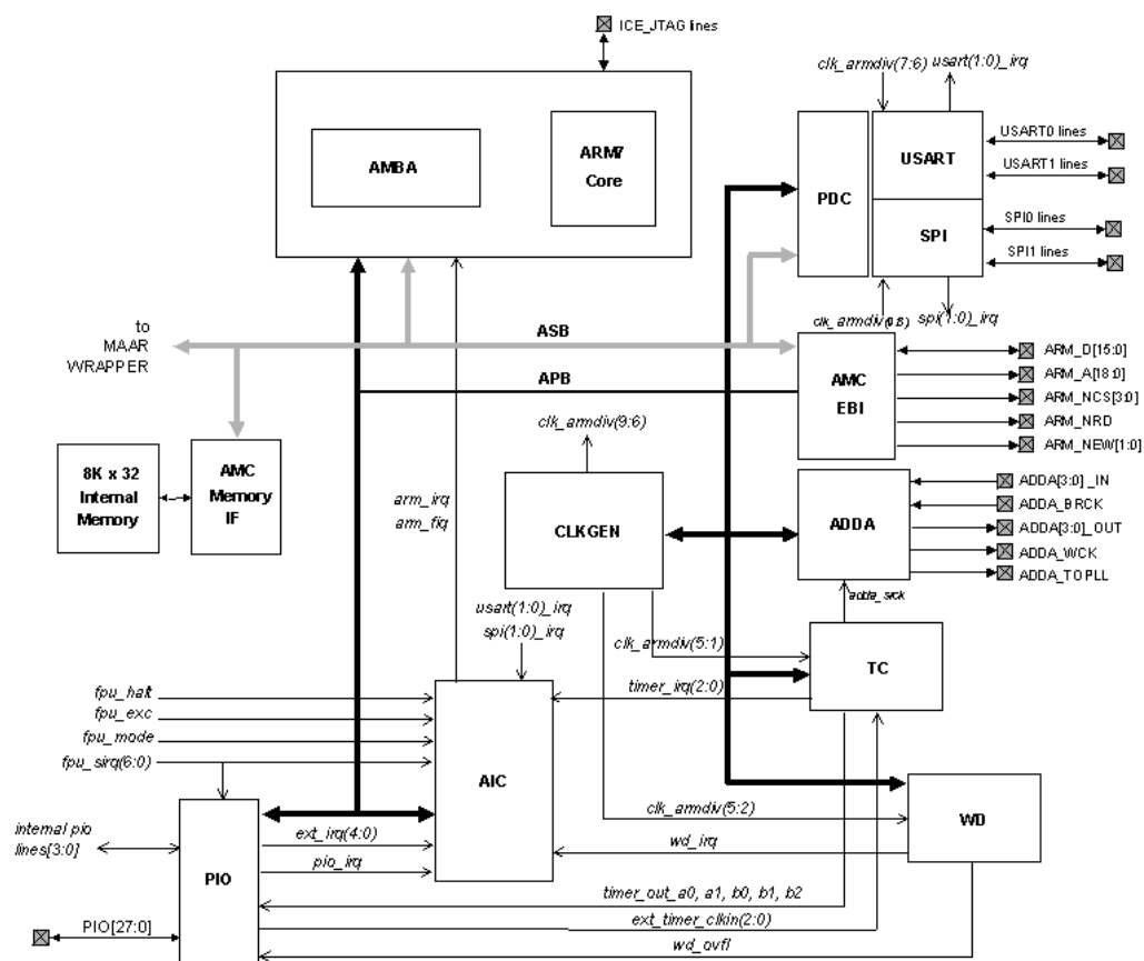
Figure 3. Armsystem Architecture
