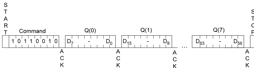
Figure 10. Initiatize Authentication
