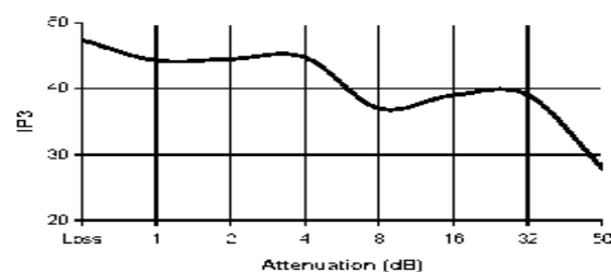
Maximum IP3 over Temperature Range and Attenuation @ 950 MHz
