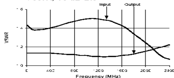
VSWR, 16 dB Bit
