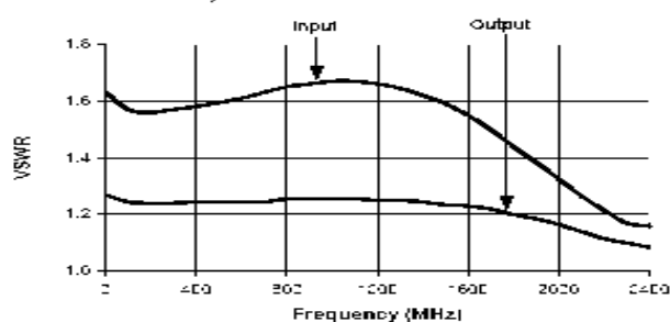
VSWR, 8 dB Bit
