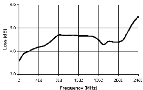
Insertion Loss
