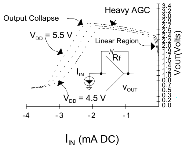
V_{OUT} vs I_{IN}
