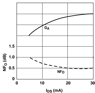
Figure 2. Optimum Noise Figure and Associated Gain vs. I DS . V DS = 2V, f = 4.0 GHz.
