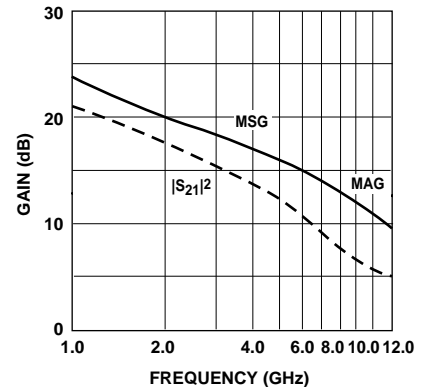
Figure 4. Insertion Power Gain, Maximum Available Gain and Maximum Stable Gain vs. Frequency. V DS = 4 V, I DS = 70 mA.
