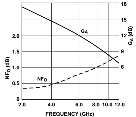
Figure 1. Optimum Noise Figure and Associated Gain vs. Frequency. V DS = 2V, I DS = 25 mA, T A = 25°C.
