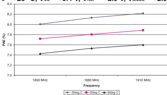
Figure 6: PAE vs. Frequency P OUT = +16 dBm, Low Bias Mode (T C = +25 °C, V CC = +3.4 V, V REF = +2.9 V, V MODE = +2.9 V)
